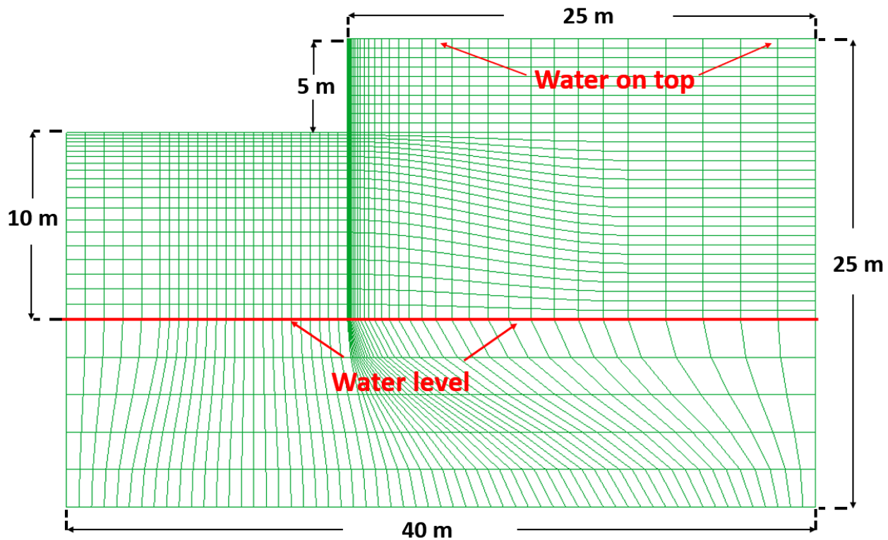
Figure 9. Boundaries for wall simulation.
