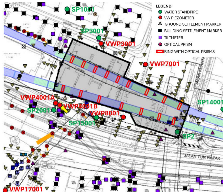
Figure 14. Instrumentation for groundwater monitoring.
