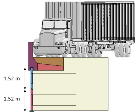
(a) Cross section of barrier-moment slab-MSE wall assembly with truck.
