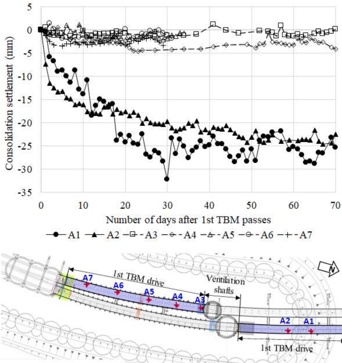
Figure 18: Tunnelling-induced consolidation settlements after 1 st TBM drive.
