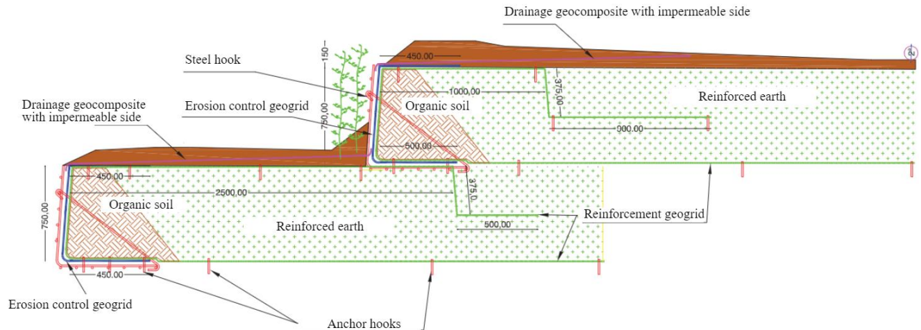
Figure 8. Cross-section of the reinforced earth wall at the berm.
