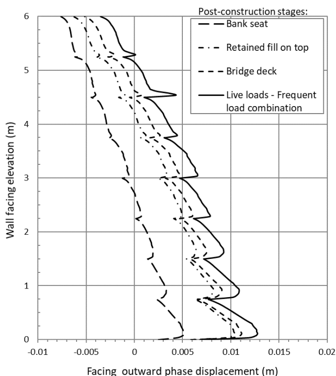
Figure 20. Facing outward displacements at post-construction wall stages.
