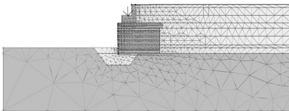
Figure 13. Construction stages after bank seat installation.
