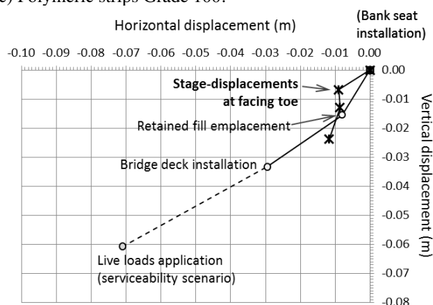
Figure 17. Displacements of the bank seat bearing center point at post-construction wall stages: (a) base case, (b) modified foundation soil properties, (c) assuming polymeric strips Grade 100, and (d) assuming steel reinforcement case. Note: (c) and (d) cases also assume modified soil properties as in b-case.
