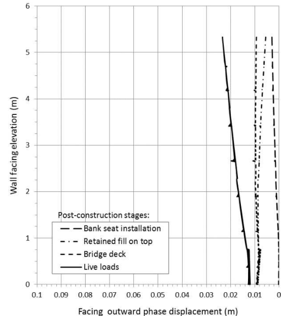
Figure 16. Facing outward displacements at post-construction wall stages: (a) base case, (b) modified foundation soil properties, (c) assuming polymeric strips Grade 100, and (d) assuming steel reinforcement case. Note: (c) and (d) cases also assume modified soil properties as in b-case.
