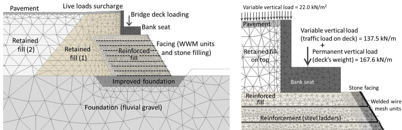
Figure 18. FEM 2D model mesh generated: (a) general model, and (b) bank seat with loading features detail.
