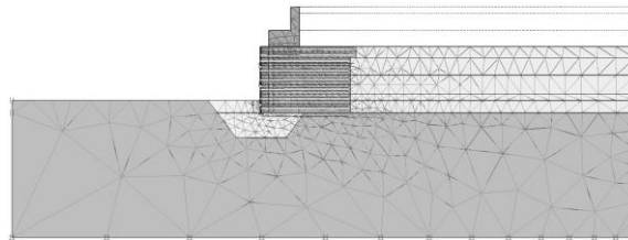
Figure 12. Construction stages up to bank seat installation.
