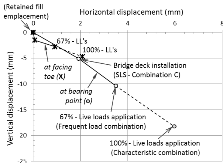
Figure 21. Displacements of the bank seat bearing center at post-construction wall stages.
