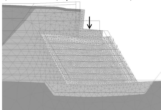
a) Deformed mesh (amplification factor: \times 200 ):
