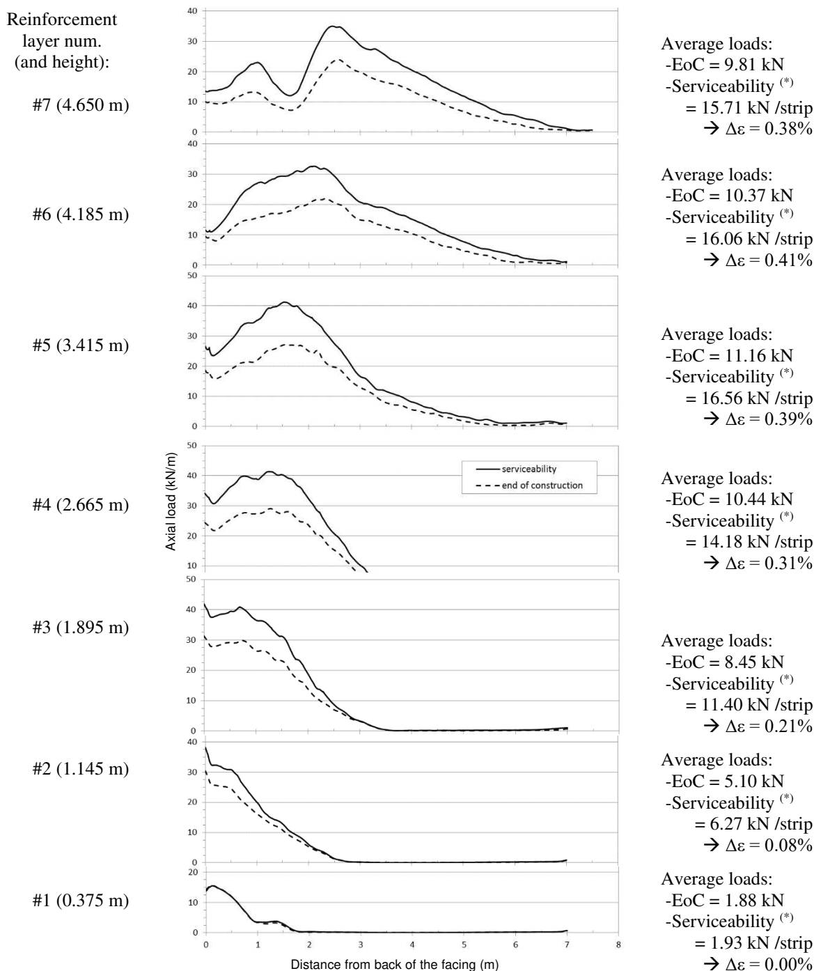
Figure 15. Reinforcement axial load (kN/m) distribution at the end of construction and under serviceability long-term scenario (*) 100% of the LL's application). Base case.
