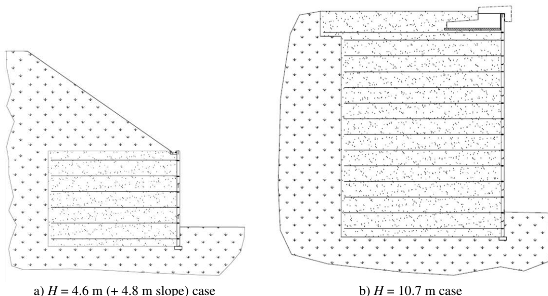
Figure 3. Simple reinforced soil wall detailed section examples: (a) with and (b) without slope on top.
