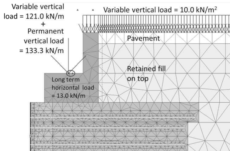
Figure 11. FE 2D model: bank seat loading features detail.
