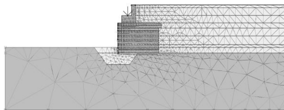
b) Bridge deck (133 kN/m permanent load surcharge at bank seat bearing center) and pavement (2 stages):
