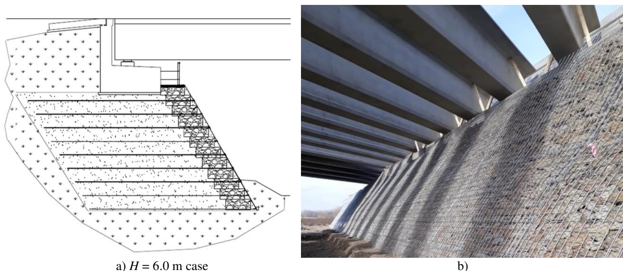
Figure 7. Bridge abutment reinforced soil slope type with WWM stone facing: (a) detailed section and (b) as-built (D4R7 Section 201-02).
