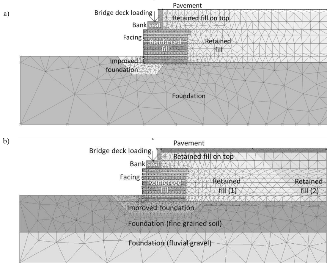
Figure 10. FE 2D model mesh generated: (a) Base case and (b) additional cases geometry.
