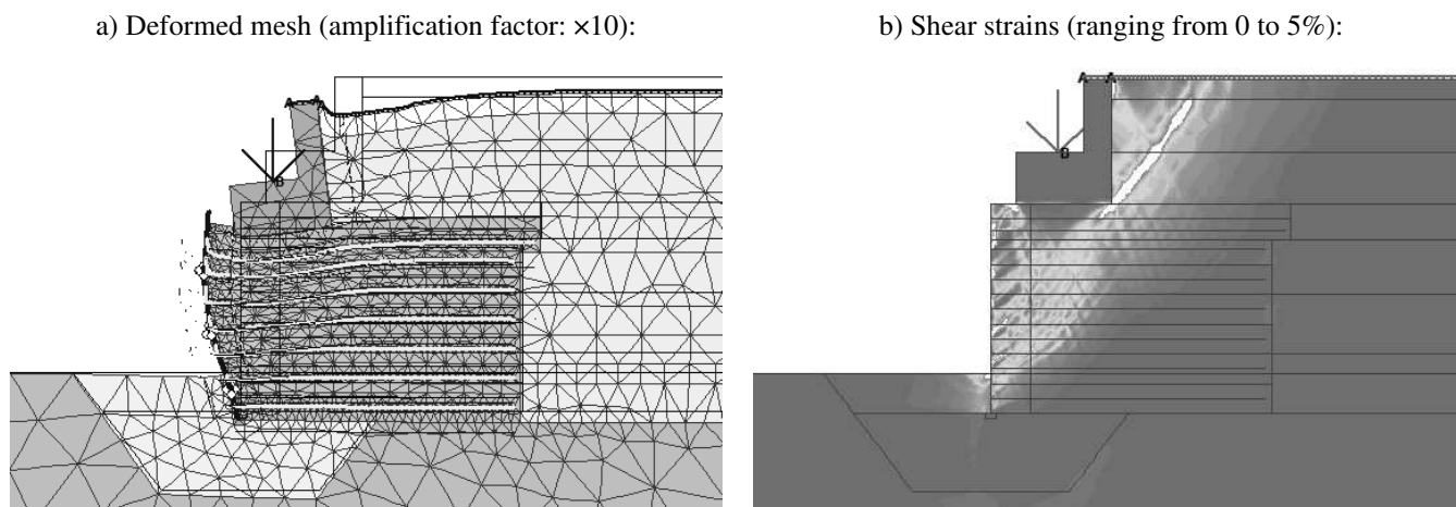
Figure 14. Deformed mesh (a) and shear strains (b) at post-construction serviceability stages. Base case.
