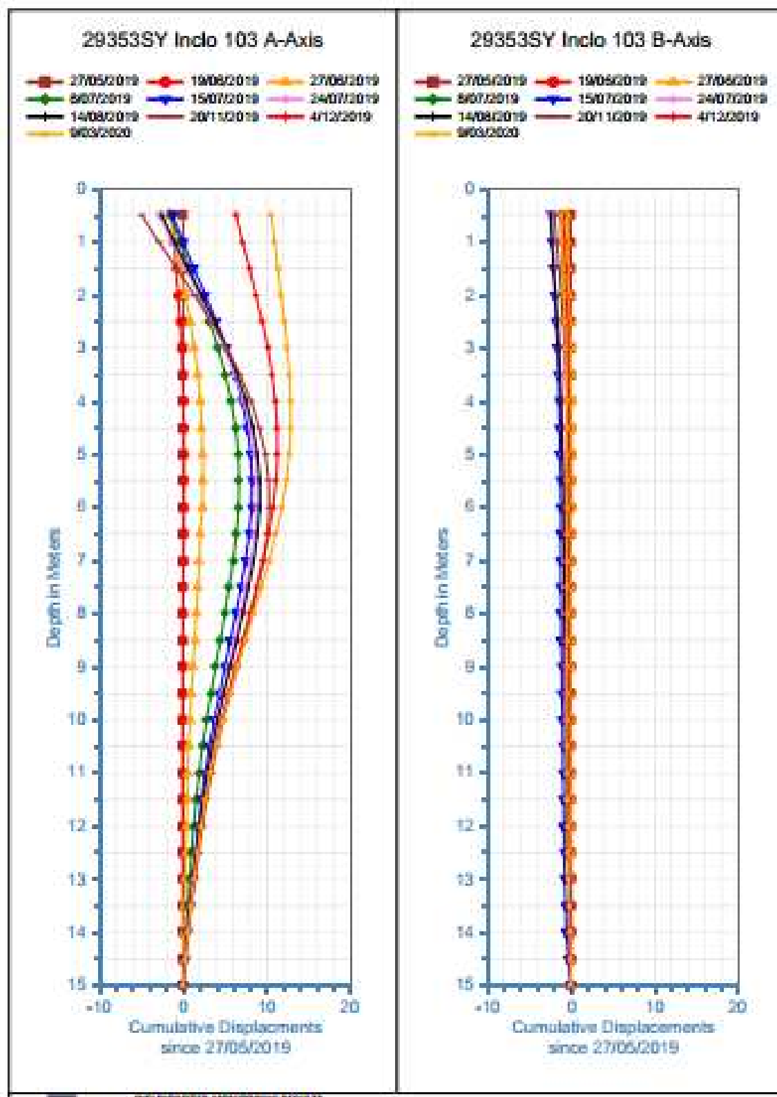
Figure 11. Inclometer 103.
