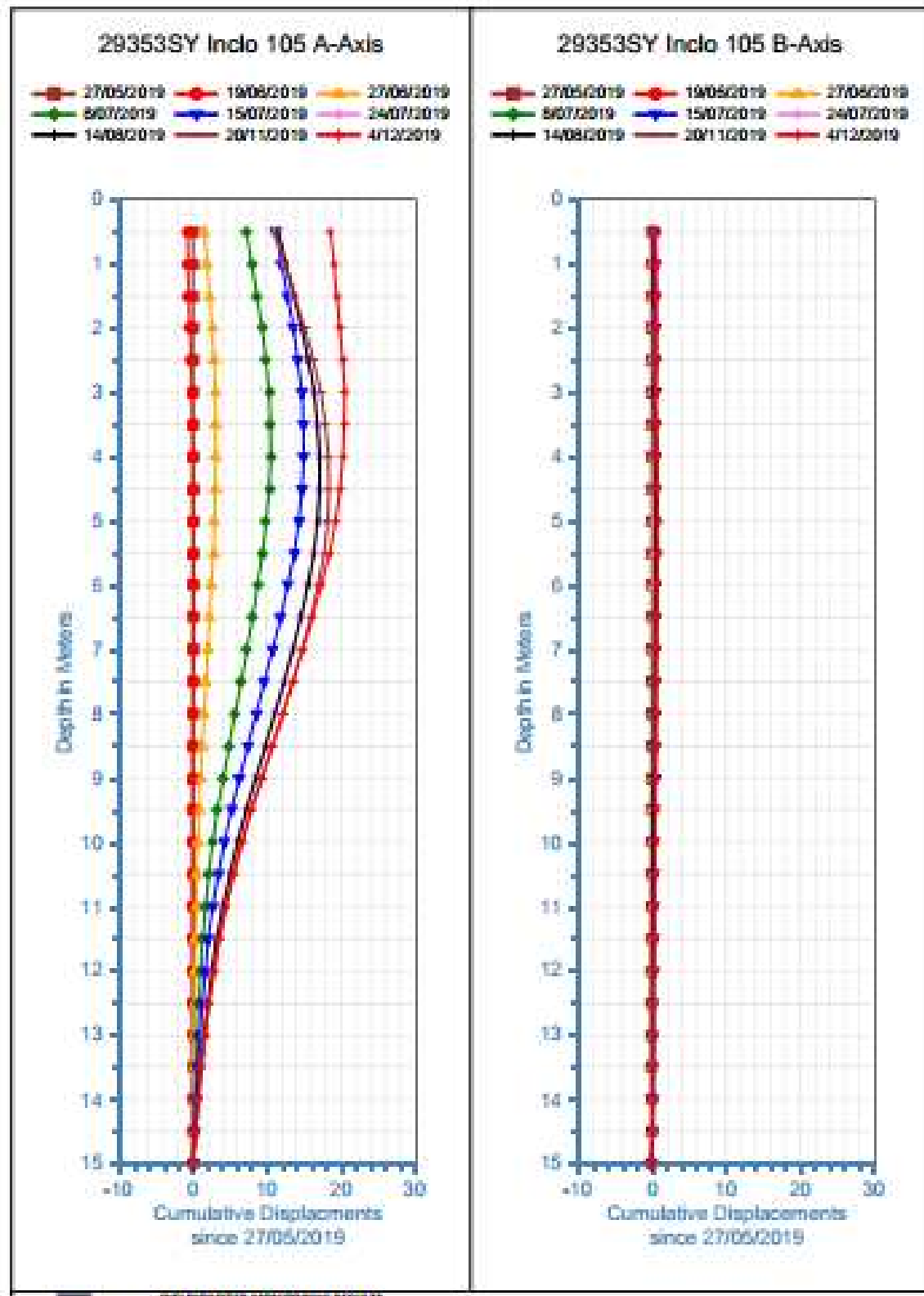
Figure 13. Inclometer 105.
