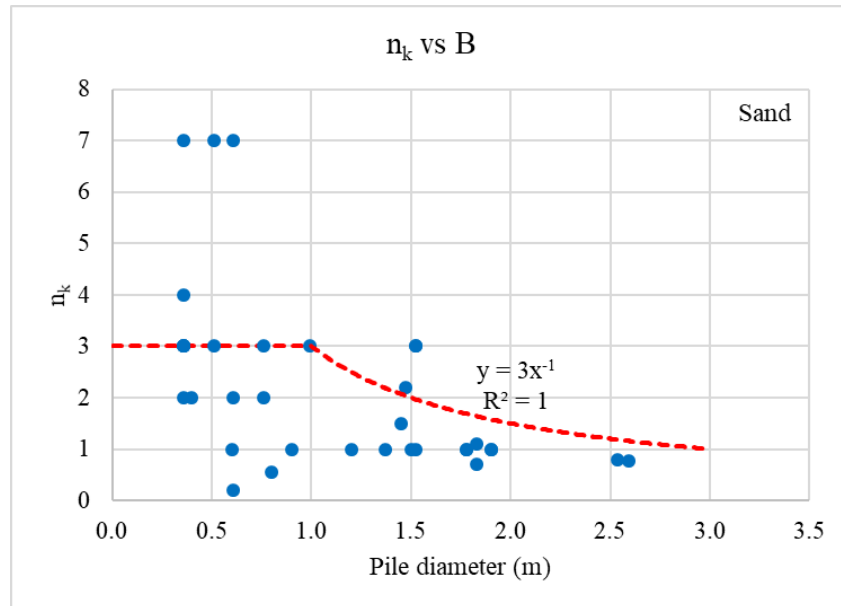
Figure 16. Correction Coefficient for the Subgrade Modulus ( n_k ) versus Pile Diameter and Proposed Curve.
