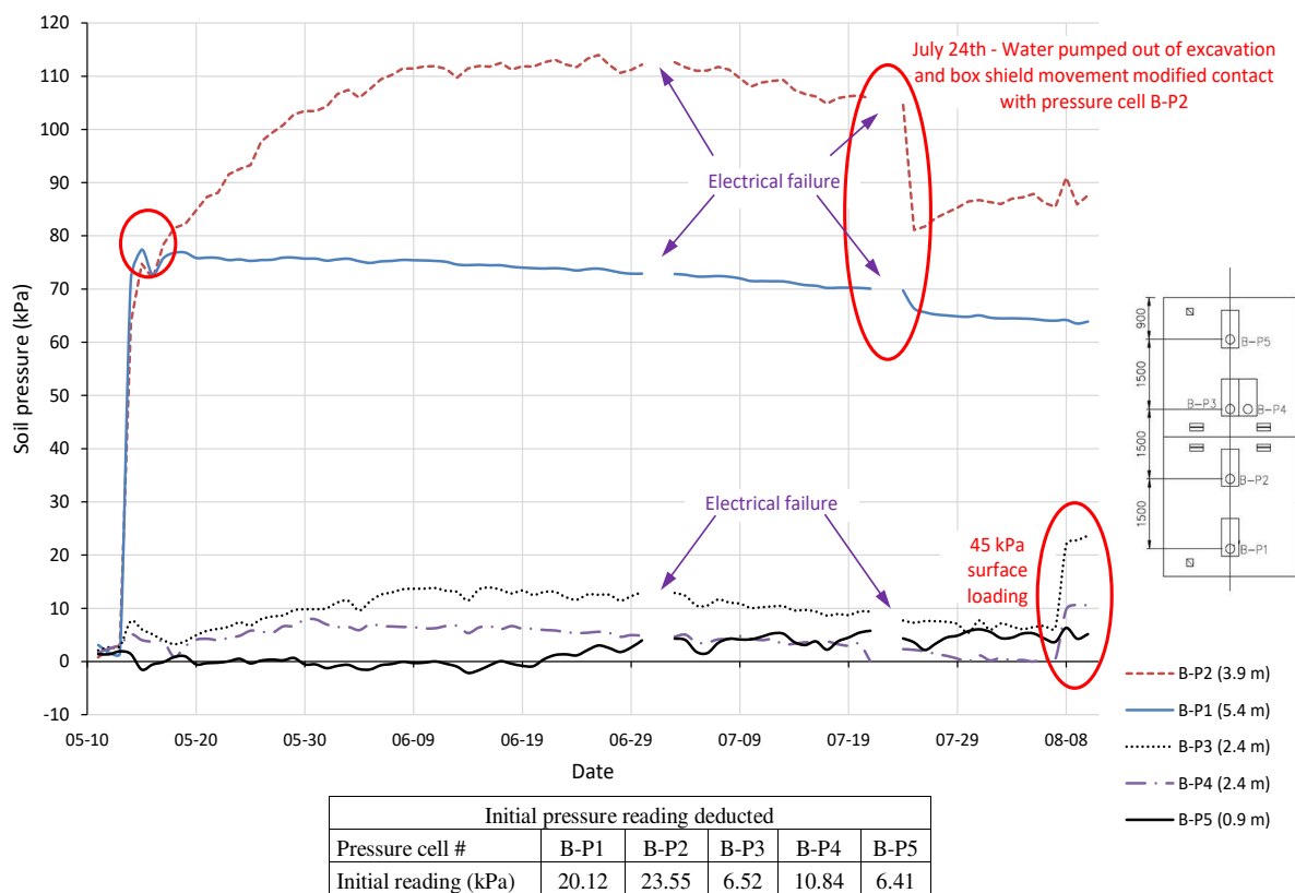
Figure 18. Maximum daily soil pressure after temperature correction on the trench box protection (May 14–August 10, 2018).
