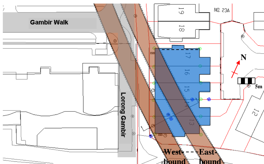
Figure .1 Layout of the 5 houses and the tunnels' alignment.
