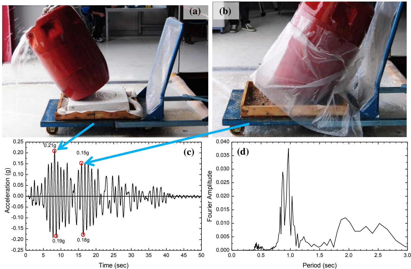
Figure 17. Results of shaking table tests on the plastic barrel-shaped container, filled with water (a) overturning of container sitting on EPS15 block, under a_{max} \approx 0.20g , (b) overturning of container sitting on silty sand layer, under a_{max} \approx 0.17g , (c) scaled acceleration time history (recorded at Patra-kiosk) used as input in the shaking table tests and (d) Fourier Spectrum of input motion.
