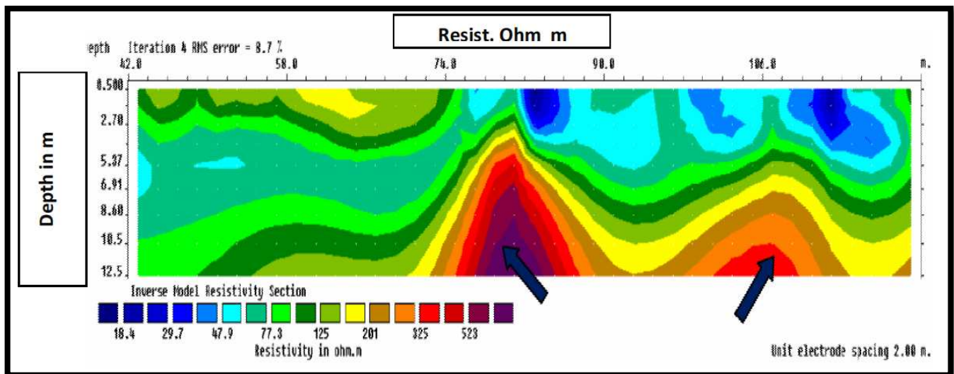
Figure 6.a. and b. Northwest part of Riyadh project using 2D electrical resistivity imaging lines A and B showing detected subsoil karst features. The marked arrows indicate high resistivity zones indicative of empty caves.
