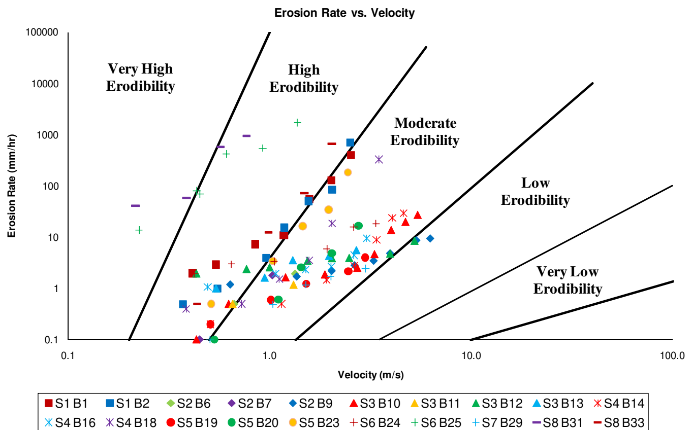
Figure 23. Erosion rate versus velocity for the Midwest Levee samples.
