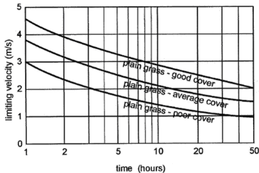
Figure 37. Limiting velocities for plain grass (Seijffert and Verheij 1998).
