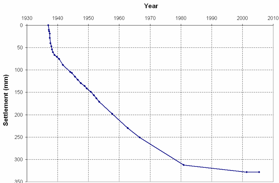
Figure 14. Settlement vs. time for San Jacinto Monument.
