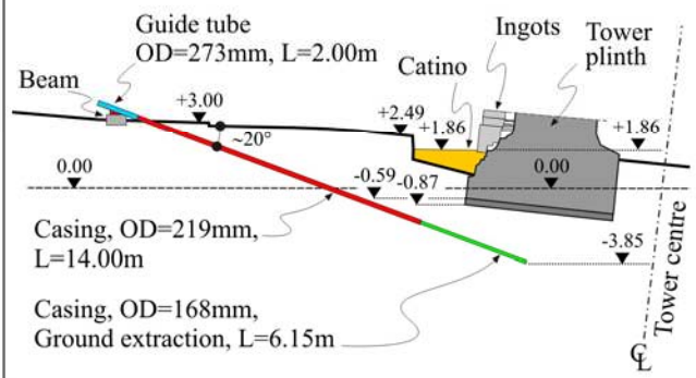
Figure 10. Holes for massive underexcavation.
