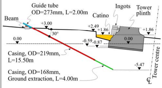
Figure 9. Holes for preliminary underexcavation.
