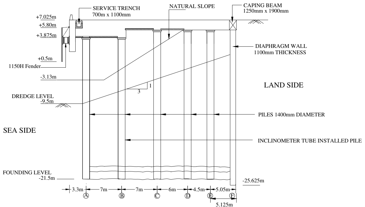
Section A-A Figure 9. Typical Cross Section of Berth.
