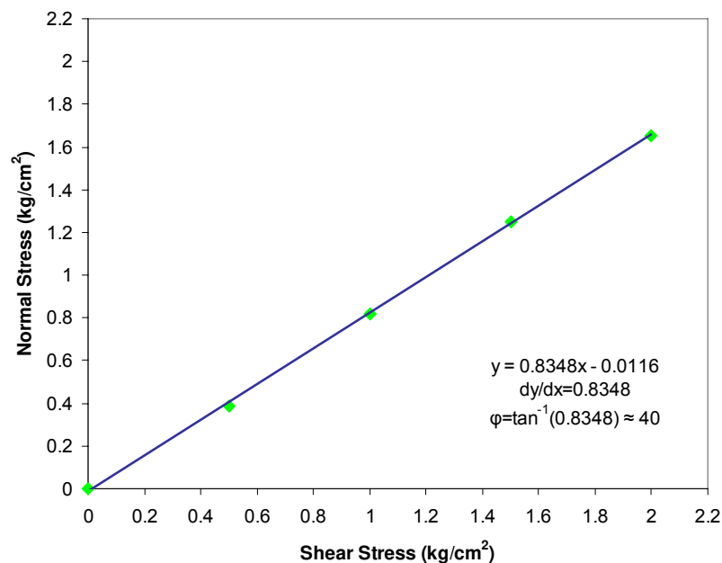
Figure 3. Direct Shear Test Result of Moorur Soil.
