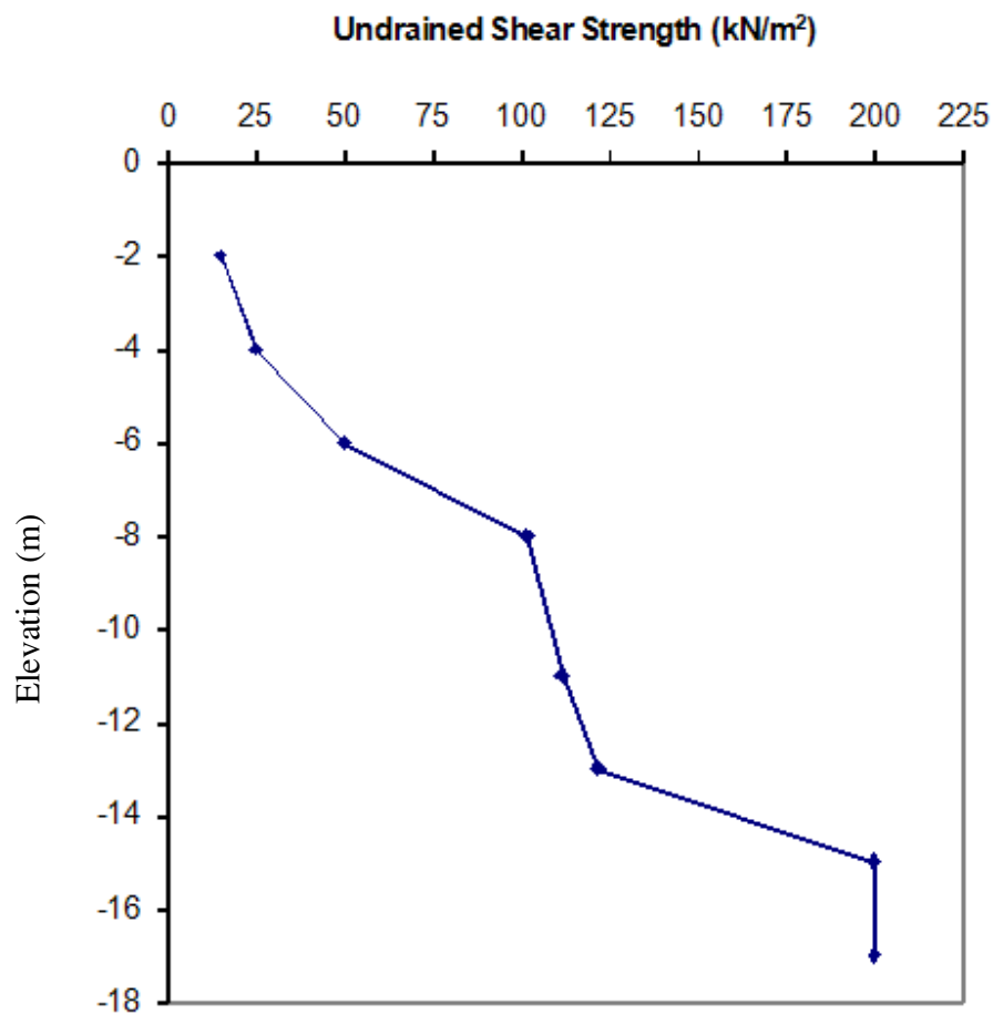
Figure 7. Variation of Undrained Shear Strength with Depth.
